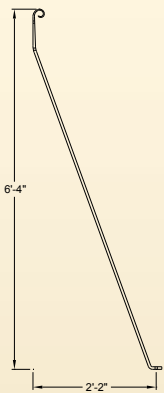
GA109 Wrought railing stay. For use with all railing panels except Stirling full height
