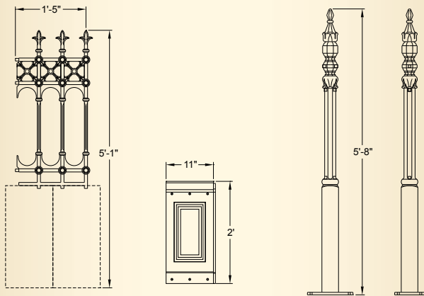
GA002 Stewart full height railing post (85lb)
