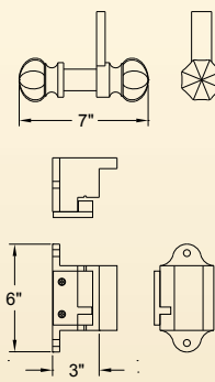
GA158 Pedestrian gate handles and striker
