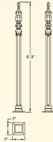
GA122 Stirling half height railing post (88lb)
