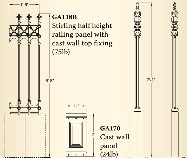
Stirling half height railing panels with cast walling system
