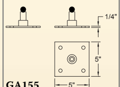
GA155 Driveway/pedestrian gate pivot (4 bolt fixing) For ground fixing
