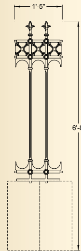
GA120B Stirling full height railing joiner panel with cast wall top fixing (60lb)
