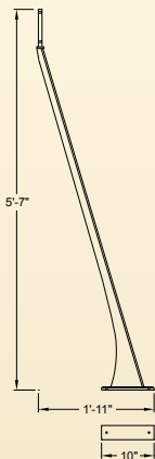
GA121 Cast full height railing stay For use with Stirling full height railing panels
