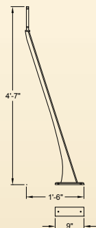
GA169 Cast half height railing stay. For use with half height railing panels
