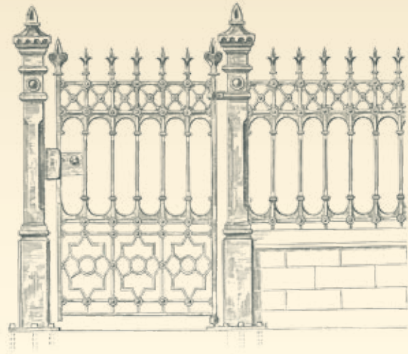
Original pattern 226a (Stewart design) 1897
