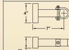
GA162 Driveway/pedestrian gate long strap hinge For use when fitting to existing pillars
