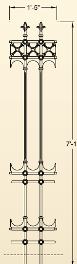
GA027 Stirling full height railing joiner panel with root fixing (90lb)
