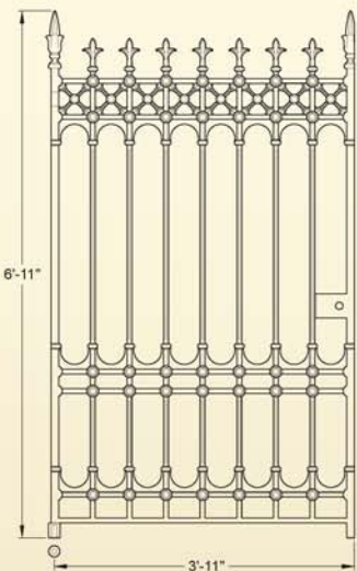
GA114 Stirling pedestrian gate (4' single gate, 391lb)
