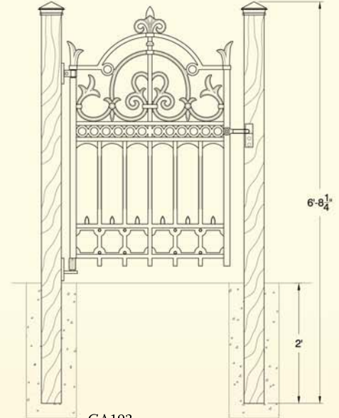
GA193 Imperial pedestrian gate with wood posts by others
