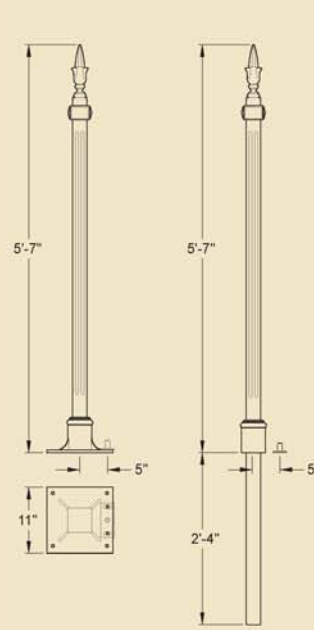
GA149 School pedestrian gate post with baseplate fixing (119lb)
