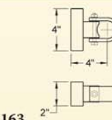
GA163 Driveway/pedestrian gate short strap hinge For use when fitting to existing pillars
