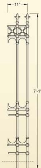
GA030 Stirling full height railing panel with root fixing (76lb)
