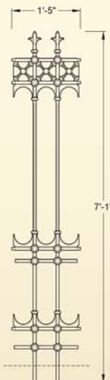
GA027 Stirling full height railing joiner panel with root fixing (90lb)
