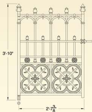
GA191 Colwyn pedestrian gate (99lb)
