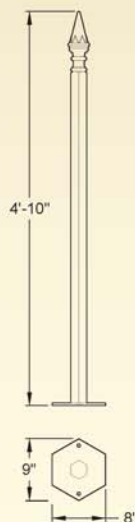
GA177 Terrace pedestrian gate post (64lb)
