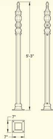
GA122 Stirling half height railing post (88lb)
