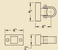
GA175 Pillar hinge and pivot set. Inc. fixing bolts
