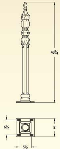
GA044 Walnut Grove 44" Post (46lbs)
