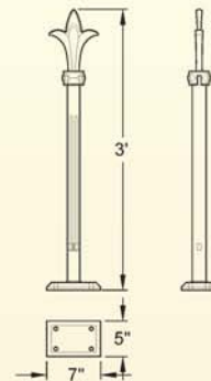
GA136 Prospect railing post (33lb)
