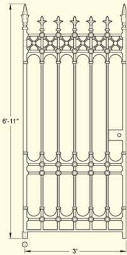
GA028 Stirling pedestrian gate (3ft single gate, 313lb)
