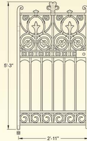
GA034 Prospect pedestrian gate (3ft single gate, 225lb)
