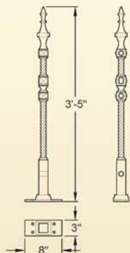
GA130 Gilberton railing post (33lb)
