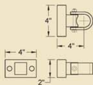
GA175 Pillar hinge and pivot set. Inc. fix- ing bolts
