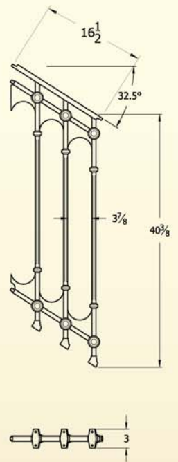
GA325 Walnut Grove Code Compliant Stair Railing @ 32.5 Degree Pitch (28.7lbs)
