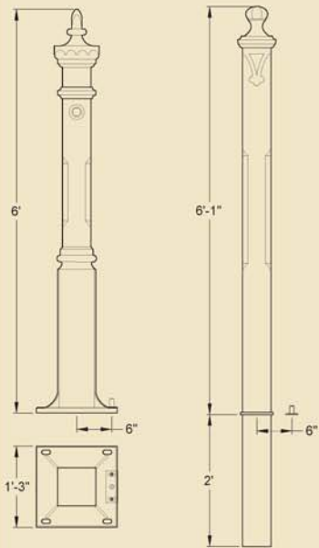
GA001 Pillar driveway gate post with baseplate fixing (268lb)
