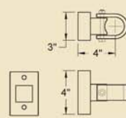
GA176 School hinge and pivot set. Inc. fixing bolts
