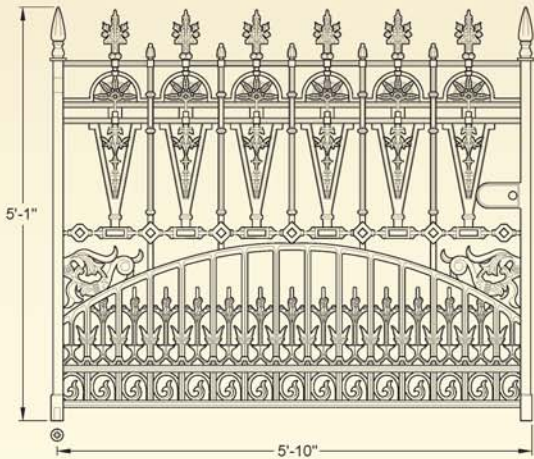
GA012 Gilberton driveway gates (12ft pair, 1023lb per pair)
