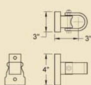
GA174 Gothic hinge and pivot set. Inc. fixing bolts
