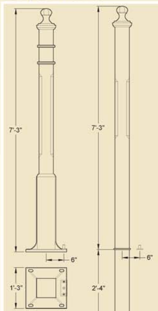
GA026 Stirling drive- way gate post with baseplate fixing (304lb)
