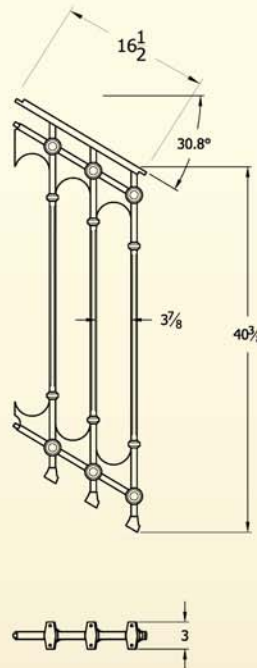
GA308 Walnut Grove Code Compliant Stair Railing @ 30.8 Degree Pitch (28.7lbs)
