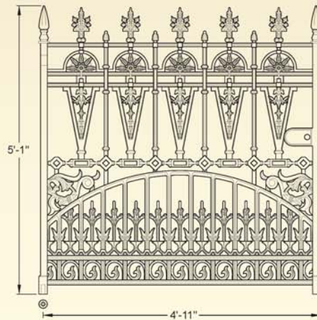
GA011 Gilberton driveway gates (10ft pair, 926lb per pair)
