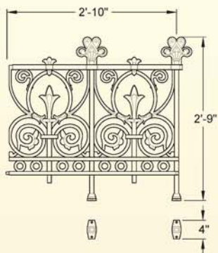
GA133A Prospect railing panel with feet (73lb)
