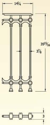
GA036 Walnut Grove 36" Code Compliant Railing (23.8lbs)
