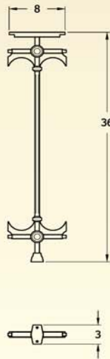
GA036J Walnut Grove 36" Code Compliant Joiner (10.4lbs)
