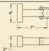
GA162 Driveway/pedestrian gate long strap hinge For use when fitting to existing pillars
