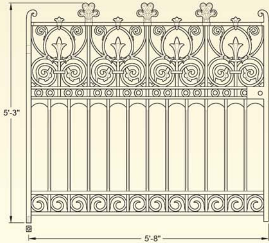
GA032 Prospect driveway gates (12ft pair, 860lb per pair)
