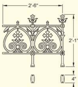
GA184 Terrace railing panel with feet (44lb)
