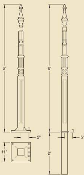
GA035 Gothic driveway gate post with baseplate fixing (209lb)
